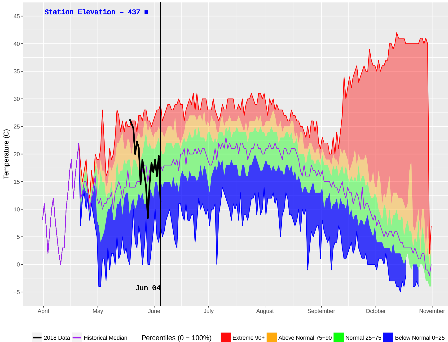
ELK MOUNTAIN (438) : Historical (1973–2016) and Current (2018) Noon Temperature
