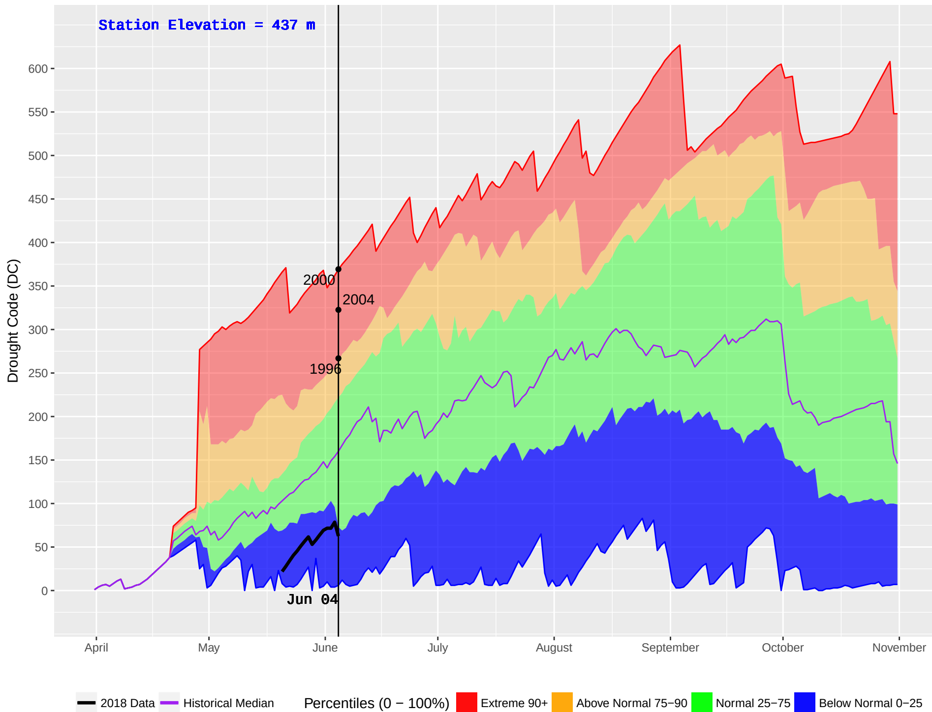
ELK MOUNTAIN (438) : Historical (1973–2016) and Current (2018) Noon Drought Code (DC)
