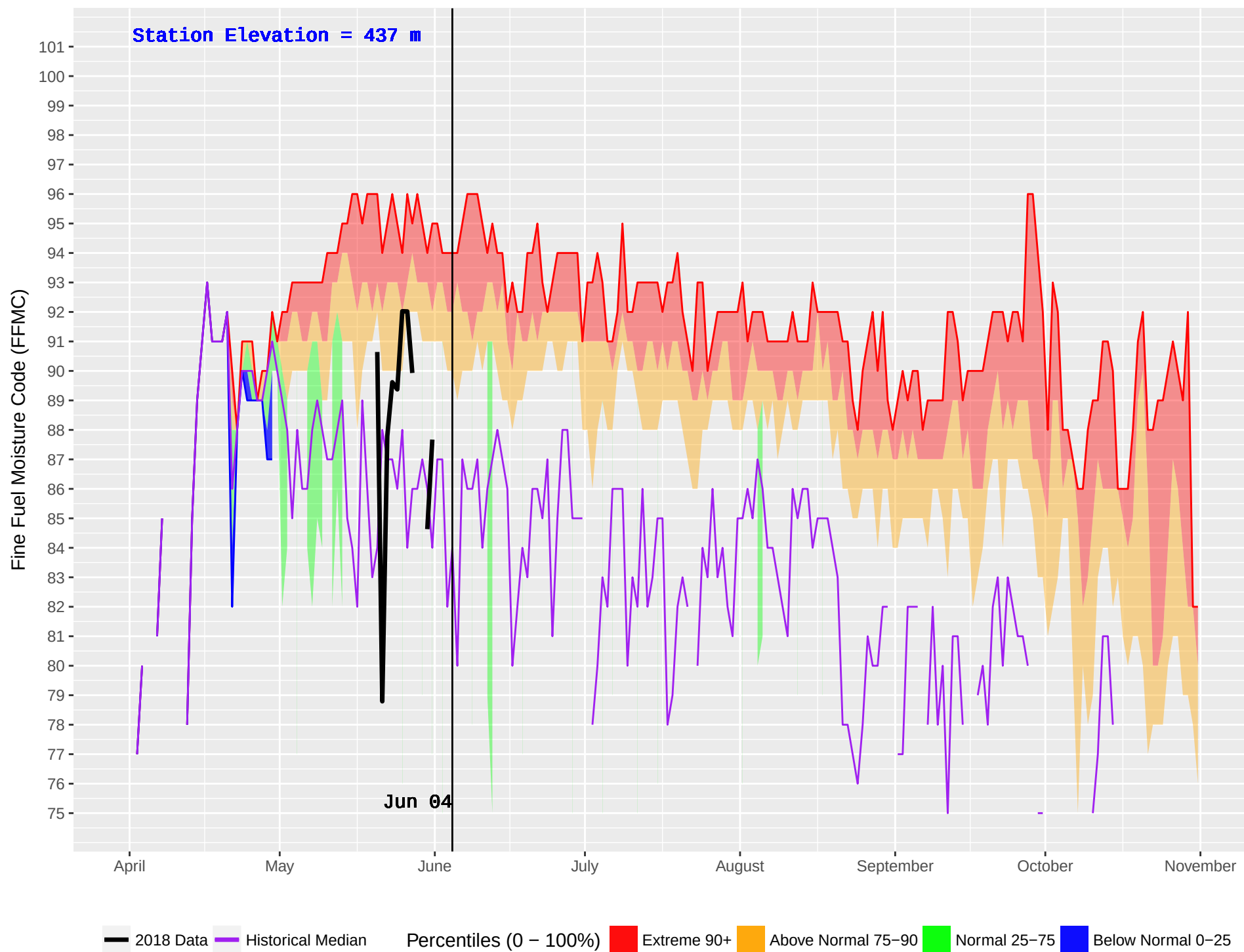
ELK MOUNTAIN (438) : Historical (1973–2016) and Current (2018) Noon Fine Fuel Moisture Code (FFMC)
